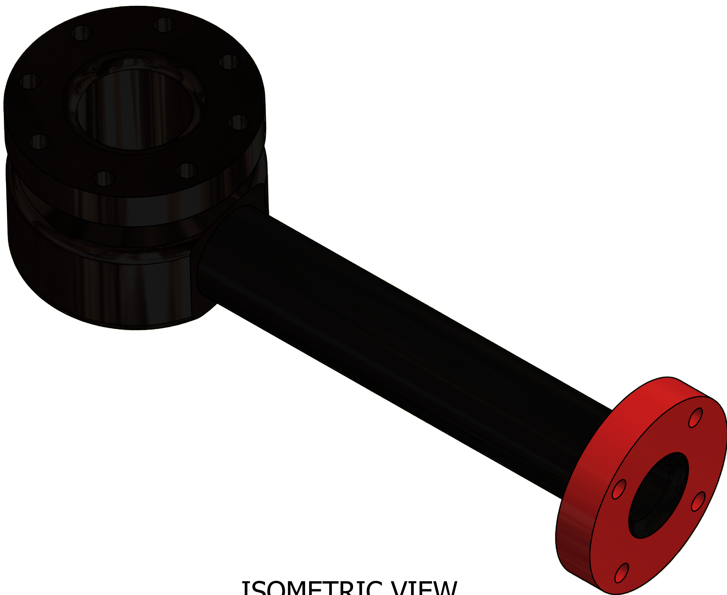
ISOMETRIC VIEW SCALE 1 : 2
