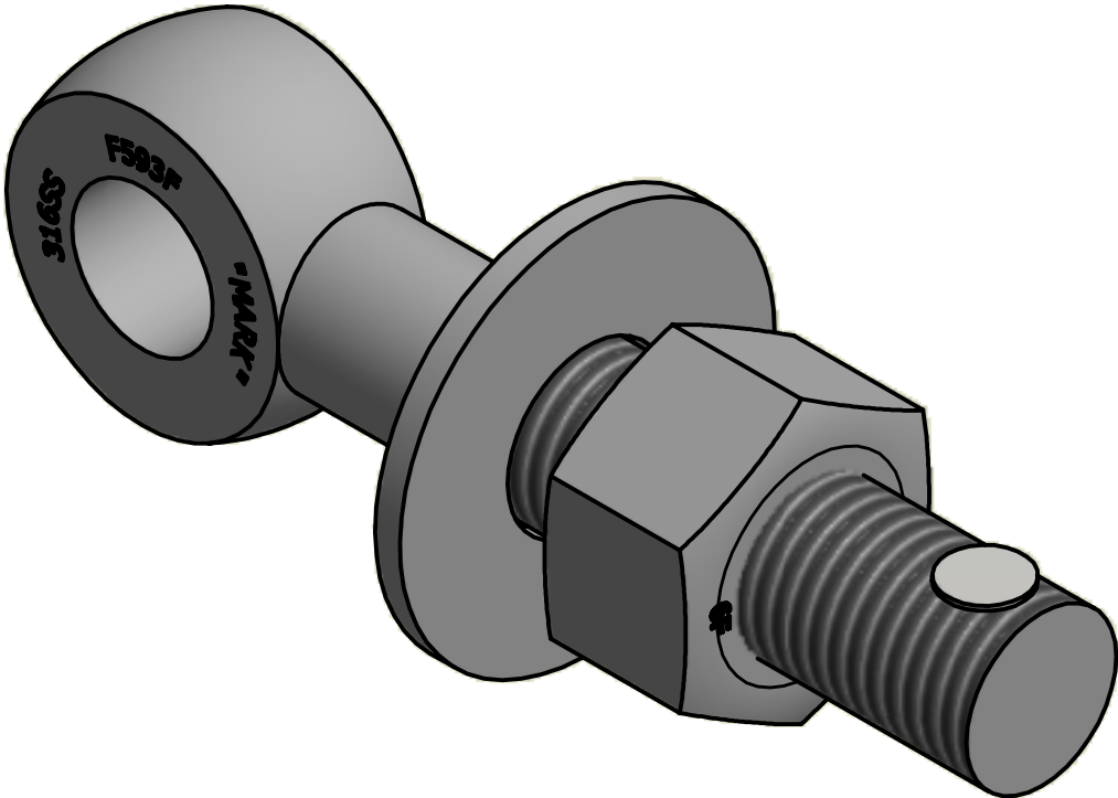
ISOMETRIC VIEW
