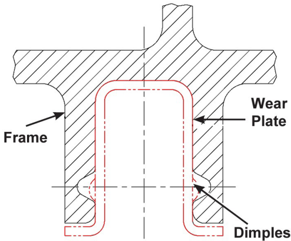
Captive Spring System
