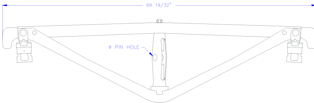
General Dimensions
